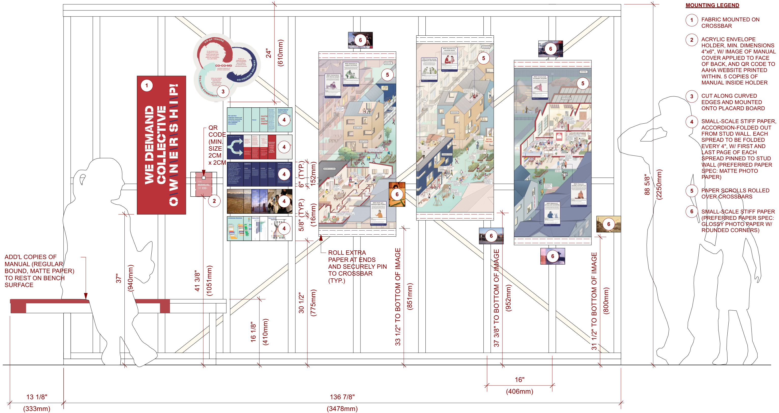
1 OVERALL STUD WALL LAYOUT 1" = 1'-0" @ 11 x 17
